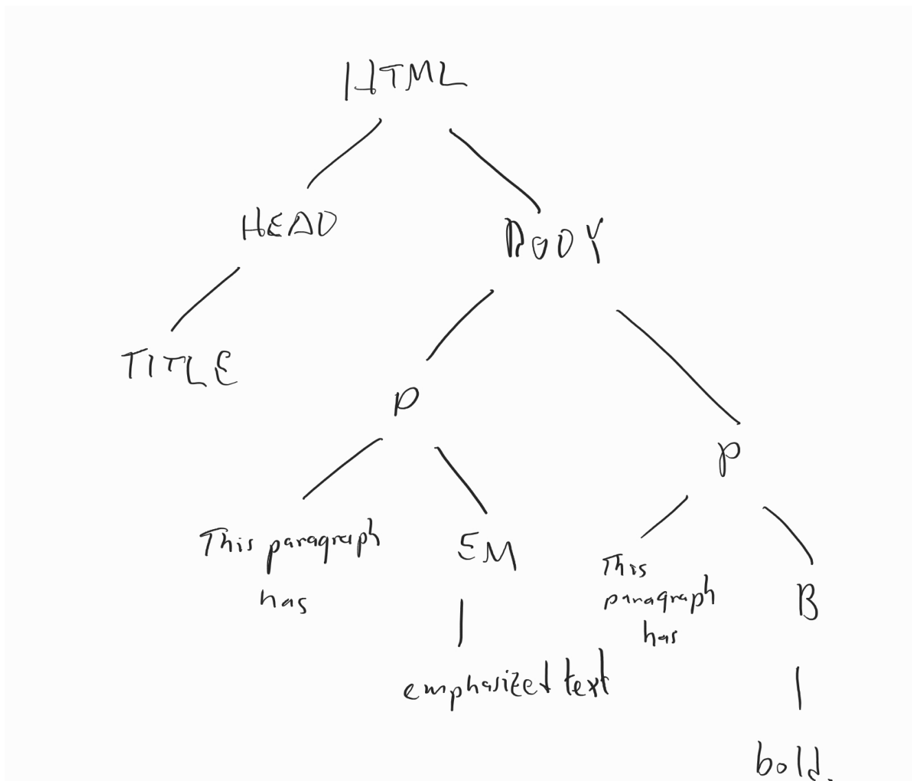
HTML tree
